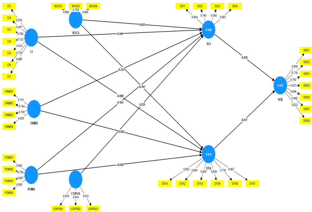
Figure.2: Measurement Model
