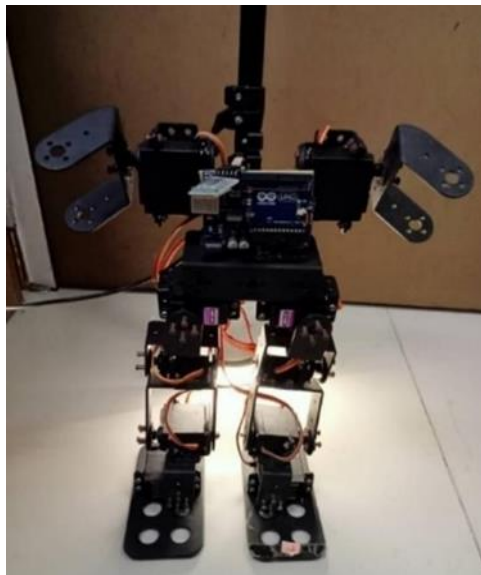
Figure 6. A prototype of a robot that incorporated blockchain technology.
