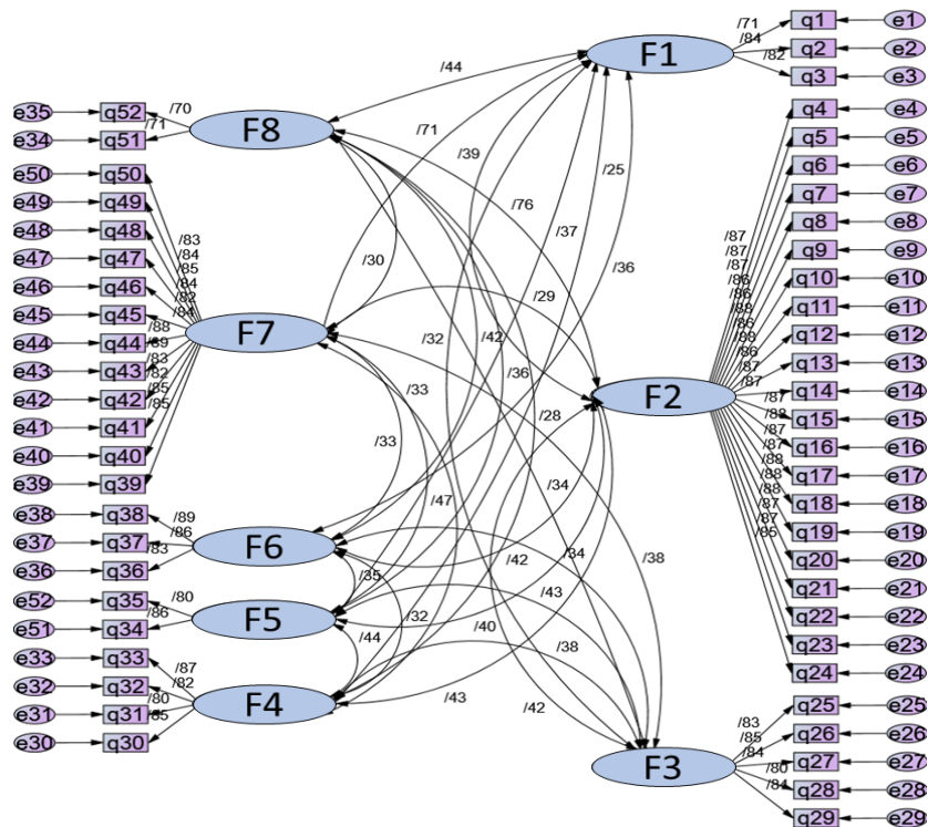
Figure.2: The First-Order Confirmatory Factor Analysis for Iran
