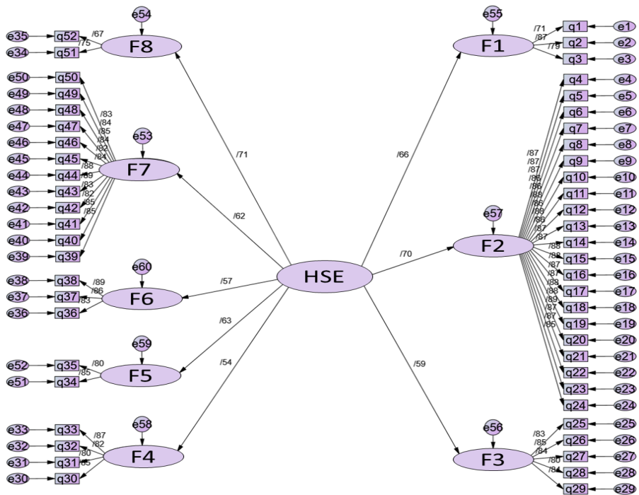
Figure.4: The Second-Order Confirmatory Factor Analysis for Iran
