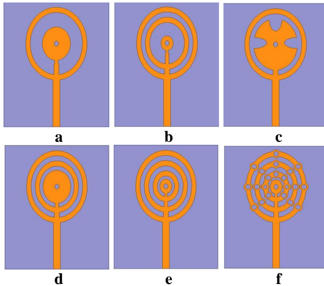
Figure 1: Illustration of the Sequential Stages involved in the Antenna Design.
