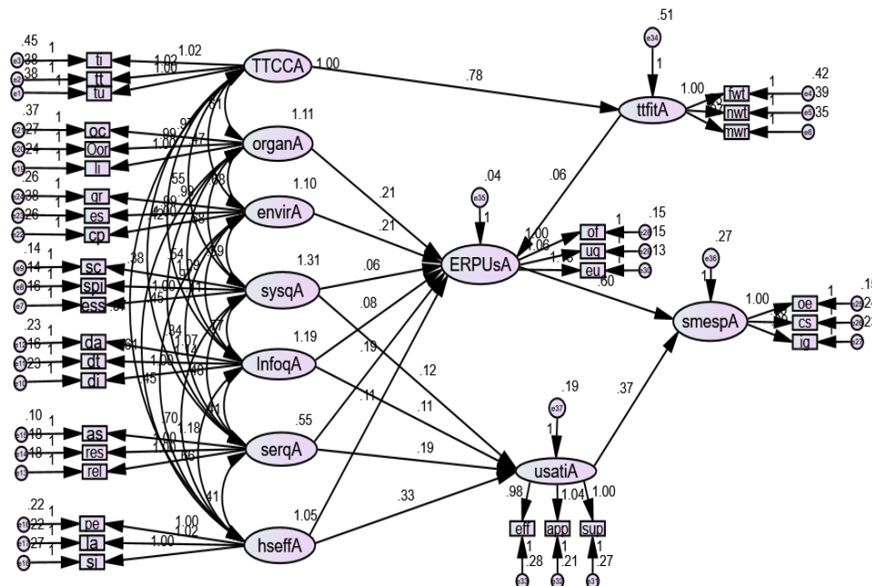
Figure 2: Empirical Model.
