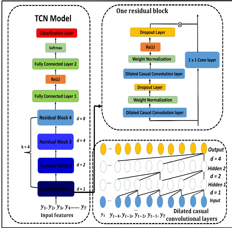
Figure 5: Entire TCN Architecture
