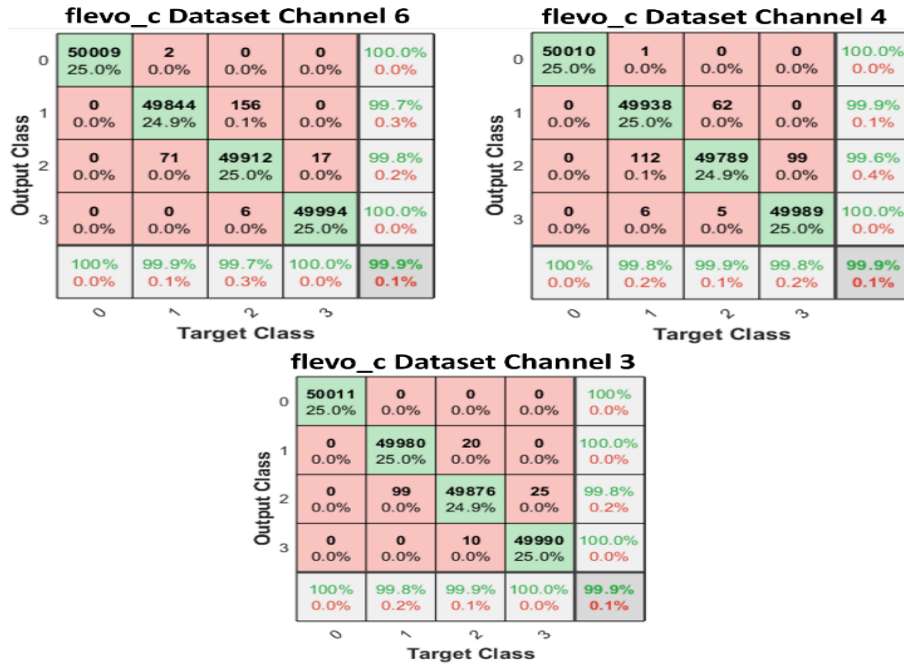
Figure 8: Flevo_l Performance using TCN Combined with SVM Classifier Based on 6, 4, and 3 Channel
