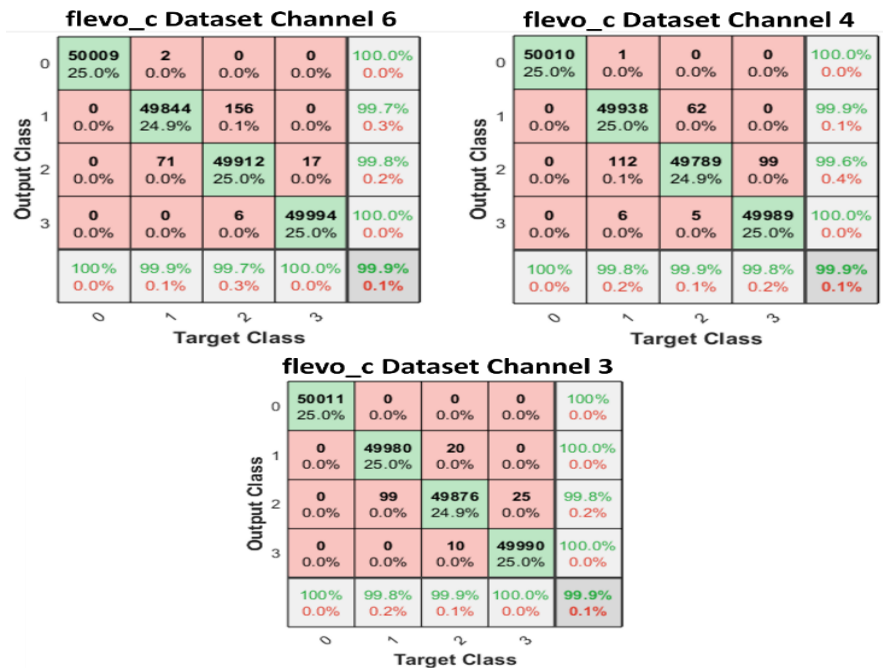
Figure 9: Flevo_c Performance using TCN Combined with SVM Classifier Based on 6, 4, and 3 Channel
