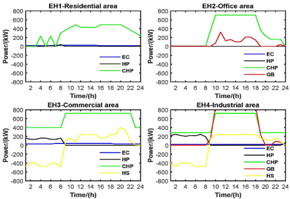
Figure 2: Operation States of Energy Converters of Energy Hub
