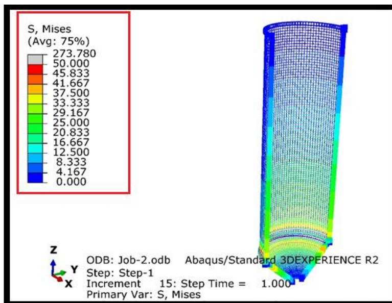
Figure 5: Model 2 Silo
